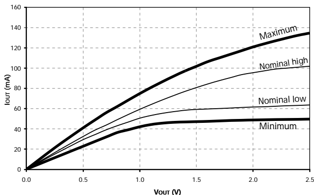
Figure 10: Pull-Down
