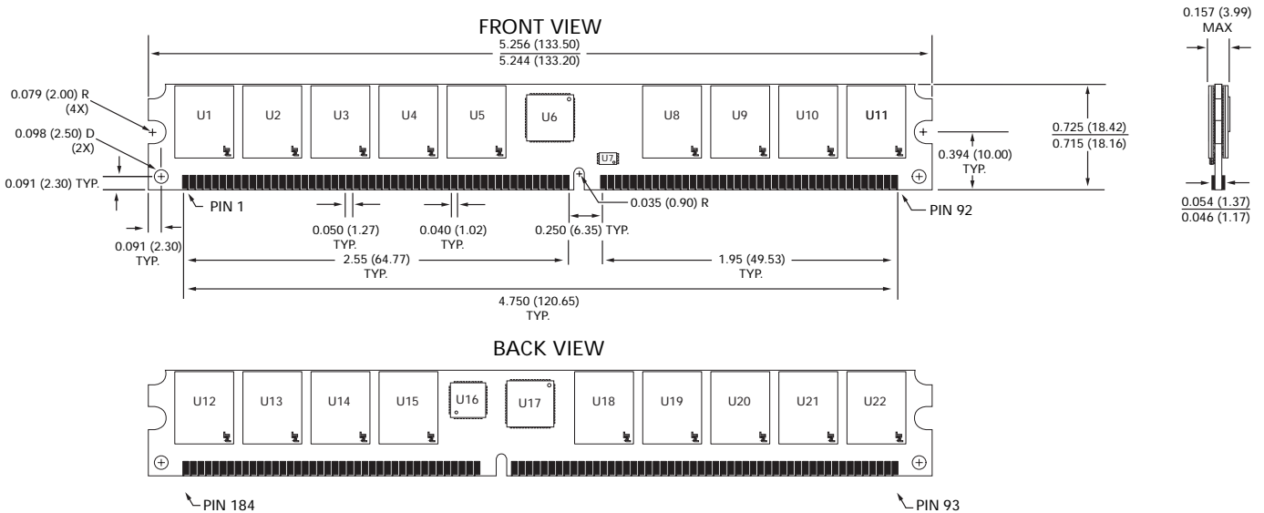
Figure 20: 184-Pin DIMM Dimensions – Very Low-Profile PCB
