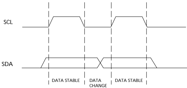
Figure 14: Data Validity
