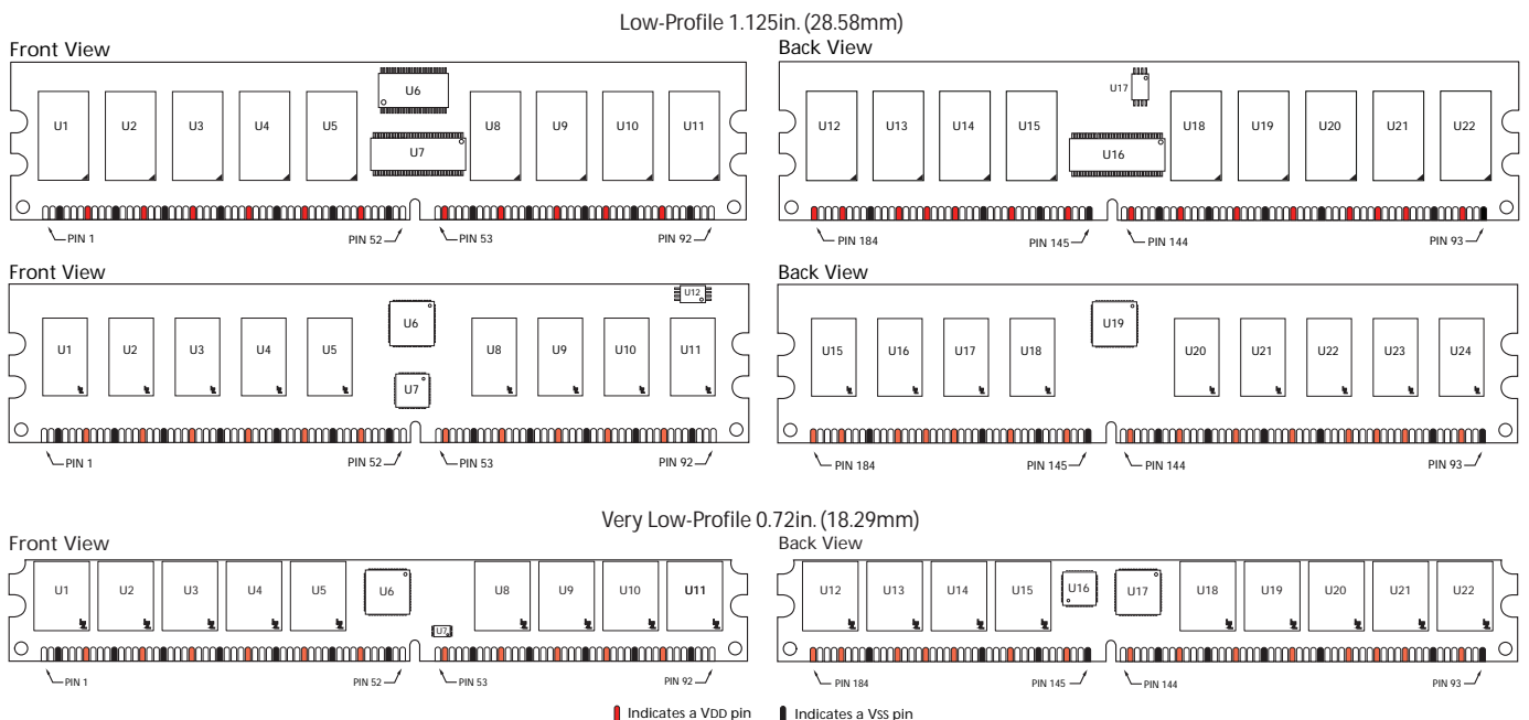
Figure 2: Pin Locations
