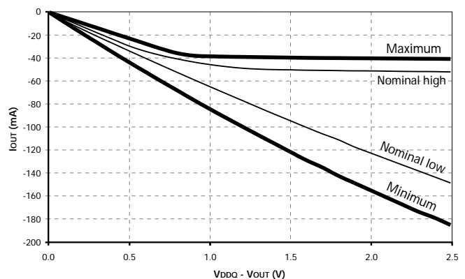
Figure 11: Pull-Up
